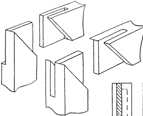
STRETCHER JOINT
